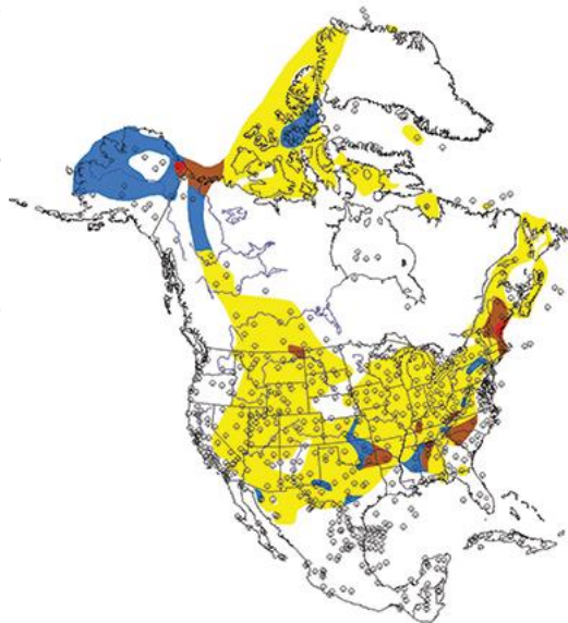
Basal Sauk (Tapeats) map of North America; yellow color represents the blanket
